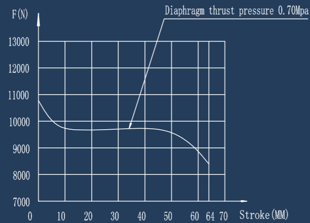
Static characteristic curve SD-24P
