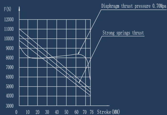
Static characteristic curve SD-S16/24PL
