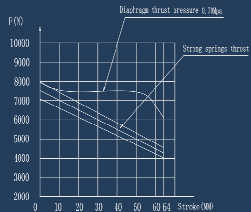
Static characteristic curve SD-16/24P
